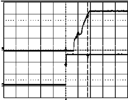
Start-up enabled by connecting V_i at: T_{ref} = +25^{\circ}\text{C} , V_i = 53\text{ V} , I_o = 50\text{ A} resistive load. Top trace: output voltage (1 V/div). Bottom trace: input voltage (20 V/div). Time scale: (10 ms/div).
