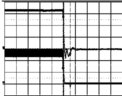
Shut-down enabled by disconnecting V_i at: T_{ref} = +25^{\circ}\text{C} , V_i = 53\text{ V} , I_o = 50\text{ A} resistive load. Top trace: output voltage (1 V/div). Bottom Trace: input voltage (20 V/div). Time scale: (0.5 ms/div).
