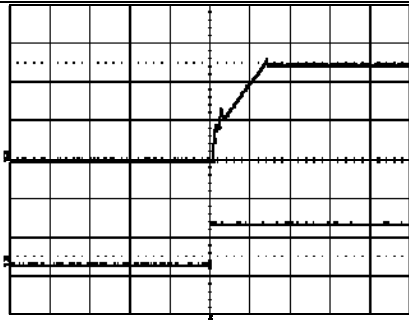
Start-up enabled by connecting V_i at: T_{ref} = +25^\circ\text{C} , V_i = 53\text{ V} , I_o = 25\text{ A} resistive load. Top trace: output voltage (5 V/div.). Bottom trace: input voltage (50 V/div.). Time scale: (50 ms/div.).
