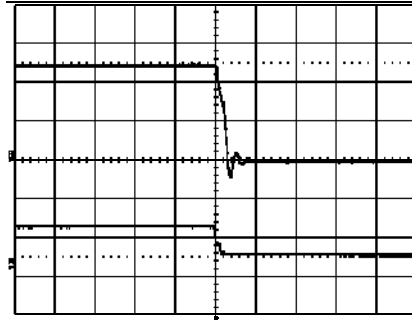
Shut-down enabled by disconnecting V_i at: T_{ref} = +25^\circ\text{C} , V_i = 53\text{ V} , I_o = 25\text{ A} resistive load. Top trace: output voltage (5 V/div.). Bottom Trace: input voltage (20 V/div.). Time scale: (0.5 ms/div.).
