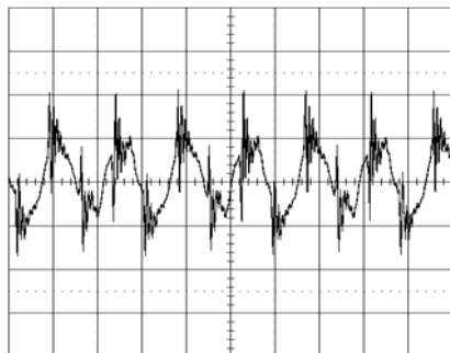
Output voltage ripple at: T_{ref} = +25^{\circ}\text{C} , V_i = 53\text{ V} , I_o = 80\text{ A} resistive load. Trace: output voltage (50mV/div.). Time scale: (2 \mu\text{s} /div.).
