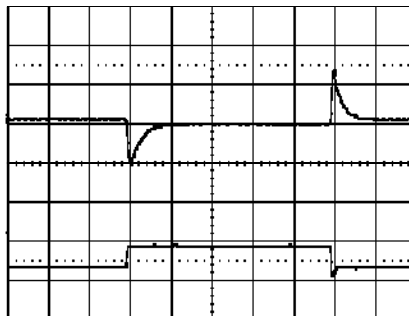
Output voltage response to load current step- Trace: output voltage (200mV/div.). change (20-40-20 A) at: T_{ref} = +25^{\circ}\text{C} , V_i = 53\text{ V} . Time scale: (0.1 ms/div.).
