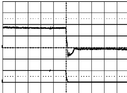
Shut-down enabled by disconnecting V_i at: T_{ref} = +25^{\circ}\text{C} , V_i = 53\text{ V} , I_o = 80\text{ A} resistive load. Top trace: output voltage (1 V/div.). Bottom trace: input voltage (50 V/div.). Time scale: (0.5 ms/div.).
