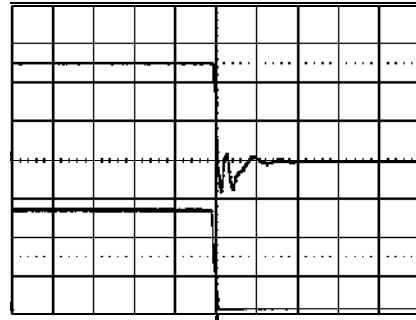
Shut-down enabled by disconnecting V_i at: T_{ref} = +25^{\circ}\text{C} , V_i = 53\text{ V} , I_o = 80\text{ A} resistive load. Trace: output voltage (1 V/div.). Bottom Trace: input voltage (20 V/div.). Time scale: (0.1 ms/div.).
