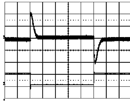
Output voltage response to load current step- change (20-40-20 A) at: T_{ref} = +25^{\circ}\text{C} , V_i = 53\text{ V} . Trace: output voltage (100mV/div.). Time scale: (0.1 ms/div.).
