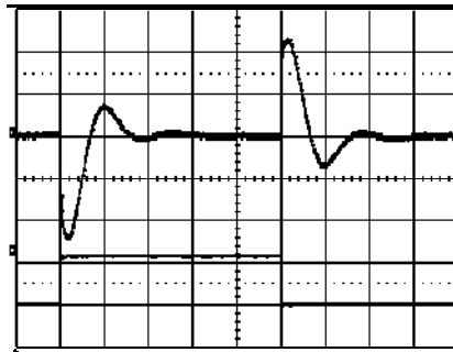
Output voltage response to load current step- Trace: output voltage (100mV/div.). change (6.25-12.5-6.25 A) at: T_{ref} = +25^\circ\text{C} , V_i = 53\text{ V} . Time scale: (0.1 ms/div.).
