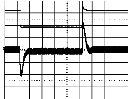
Output voltage response to load current step- Trace: output voltage (100mV/div). change (12.5-25-12.5 A) at: T_{ref} = +25^{\circ}\text{C} , V_i = 53\text{ V} . Time scale: (0.1 ms/div).
